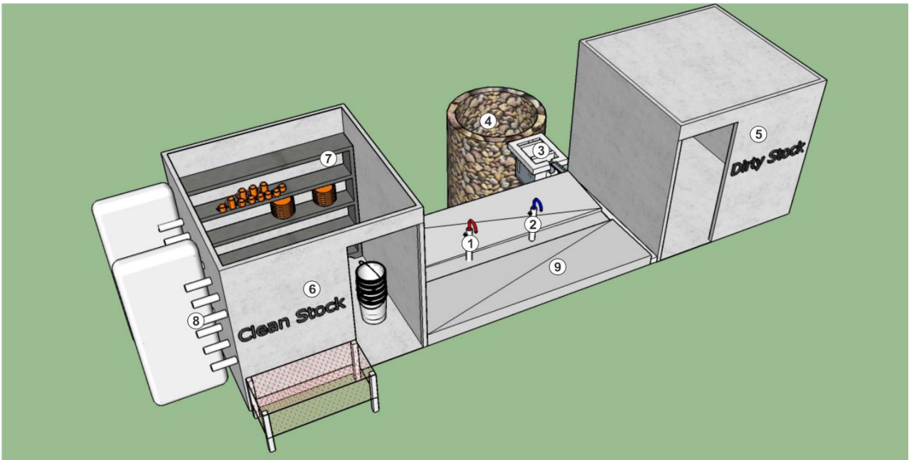
1. 0.5% Chlorine solution tap, 2. Clean water tap, 3. Grease tap, 4. Soak away or infiltration trenches, 5. Store room for contaminated material, 6. Store room for clean material, 7. Drying rack for plates, buckets, 8. Drying rack for mattresses, Shelves to store clean materials, 9. Slope
